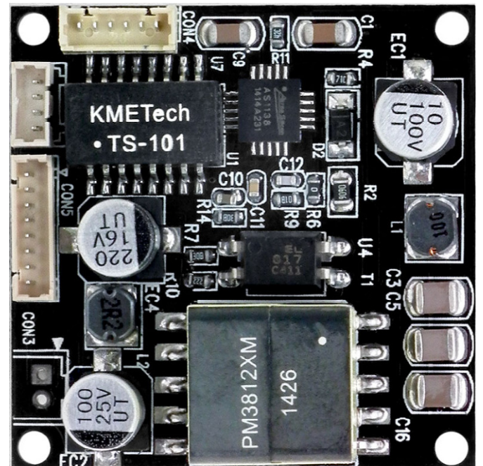
POE BOARD
